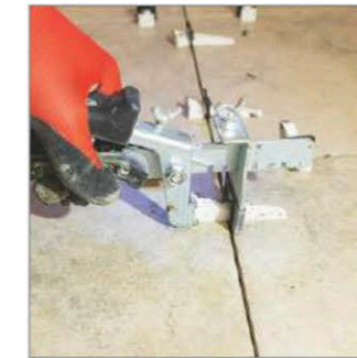
Lavelling Wedges
